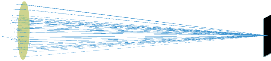
Fig. 1. A segment of the direct Cherenkov light detector with 400 \text{ cm}^2 total area. The detector will have 7 or 19 such lenses with a single sensitive element in its focus.
