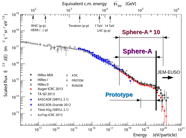
Figure 2. The energy range of the experiment Sphere-Antarctica.
